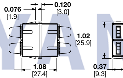
SC Duplex Adapter
